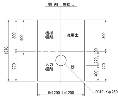
仮土工-4 (不断水T字管)
